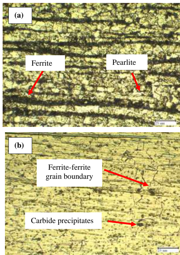
Figure 10: (a) Optical micrograph of the as-received low carbon steel (b) Optical micrograph of the as-received SS stainless steel.
