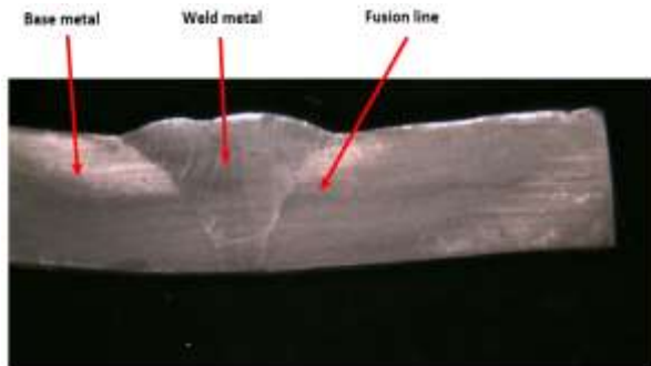
Figure 4: Macroprofile of stainless steel welded at heat input of 1250 J/mm,
