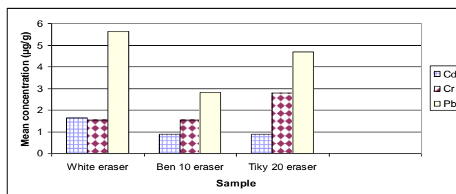
Figure 3: Distribution of cadmium, chromium and lead in the eraser brands from AAS.
