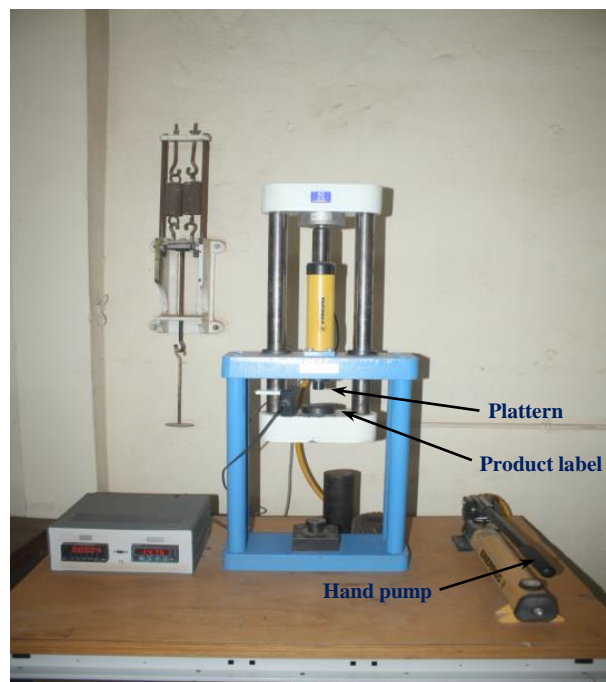
Figure 1: Universal material testing machine on a desk.
