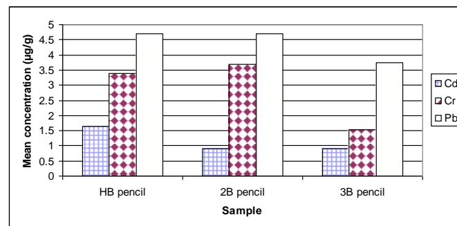
Figure 2: Distribution of cadmium, chromium and lead in the pencil types from AAS.
