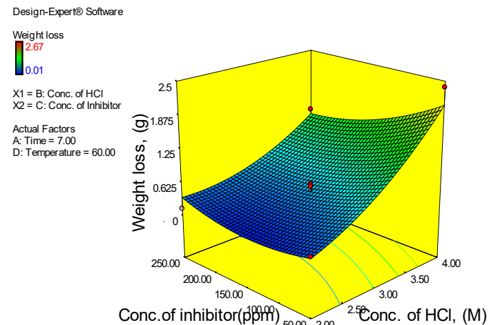
Figure 7: The effect of HCl concentration, inhibitor concentration, and boundary by weight loss plot.
