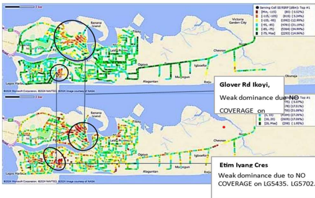
Figure 7 5G DL PLOT: SS-RSRP & SS-SINR
