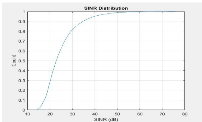
Figure 10 SINR values experienced by the User
