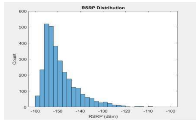
Figure 12 RSRP Distribution
