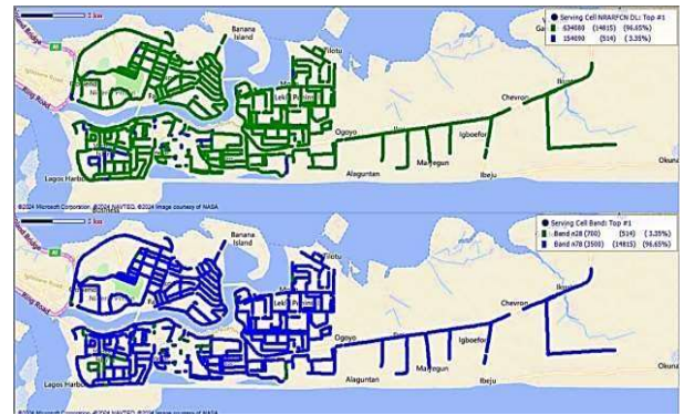
Figure 5 5G Downlink Plot (FREQUENCY and BAND)
