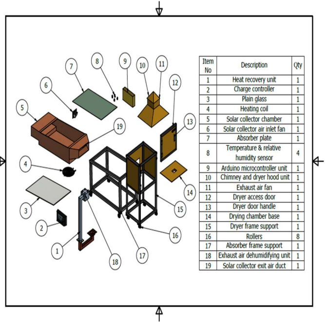
Figure 3: The exploded view of the SDED.
