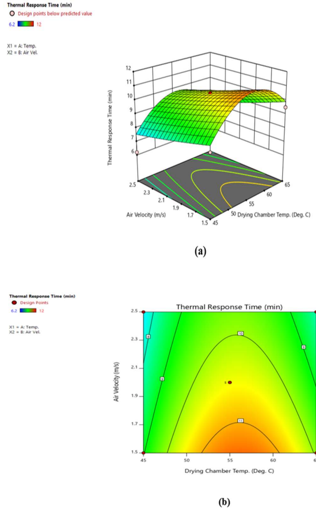
Figure 7: Response surface and contour plots of the impact of drying chamber preset temperature and air speed on heat start-up time in SDED.
