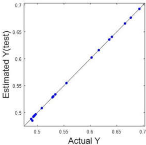
Figure 4. Correlation cross-plot for testing dataset: impact attenuation rate of 3D printed hip protection between estimated and experimental values
