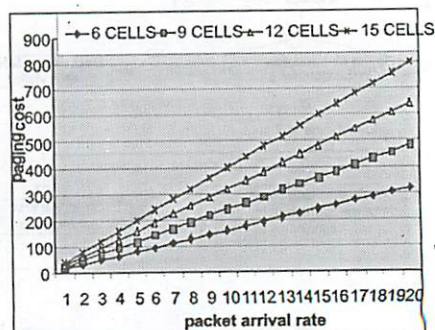
Fig.5 Effects of varying the size of a paging area in the UADP
